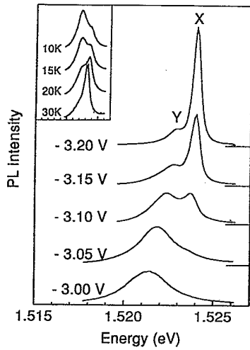
FIG. 1. PL spectra of the sample with 200 Å well and 150 Å spacer at 4 K for different gate voltages. The inset shows the PL spectra at different temperatures at V_g = -3.075 V.
