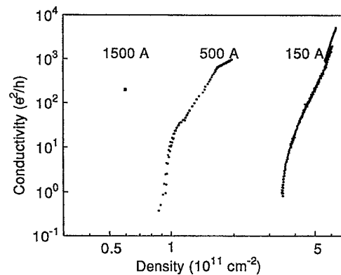
FIG. 3. The conductivity (in units of e^2/h ) versus the 2DEG density for the 150 and 500 Å spacer samples. The curves are obtained by a four probe Hall measurement with B = 0.1 T. The result of a measurement at V_g = 0 for the 1500 Å spacer sample is also shown.
