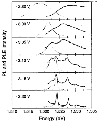
FIG. 4. PLE (solid) and the corresponding PL (dots) spectra for the sample with 200 Å well and 150 Å spacer at different gate voltages. The detection energy is 1.5187 eV.
