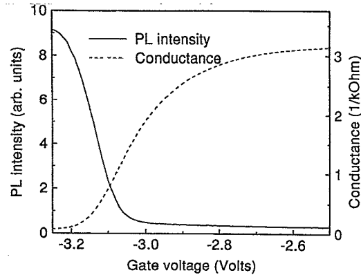
FIG. 2. PL intensity at the exciton energy position of 1.524 eV and conductance versus gate voltage for the sample with 200 Å well and 150 Å spacer. The upper value of the conductance is limited by the contact resistance, which is \sim 300 \Omega . The leveling of the conductance curve for V_g < -3.1 V is caused by gate leakage of the large area device used for optical measurements.
