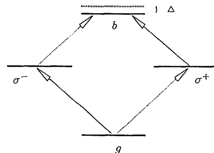
FIG. 1. The four-level system consisting of a ground state g , two exciton states \sigma^\pm , and a biexciton state b with a binding energy \Delta .
