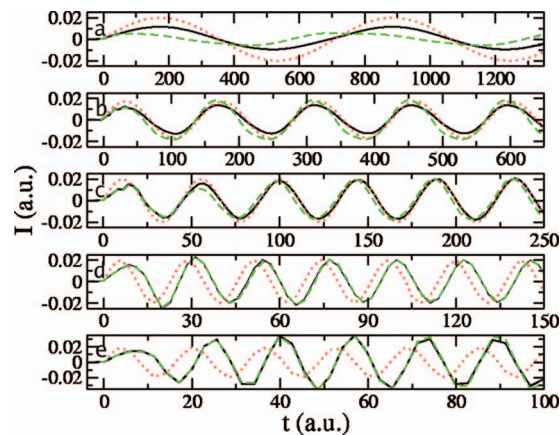
FIG. 7. Current as a function of time for H_2 molecules subjected to ac signals of varying frequencies, smaller to higher from panels (a) to (e). A well-coupled case (solid, d1=1.5 Å) and weakly coupled case (dashed, d1=2 Å) are compared to the applied voltage (dotted, 1 V amplitude). The interatomic distance in the leads is 1.5 Å.
